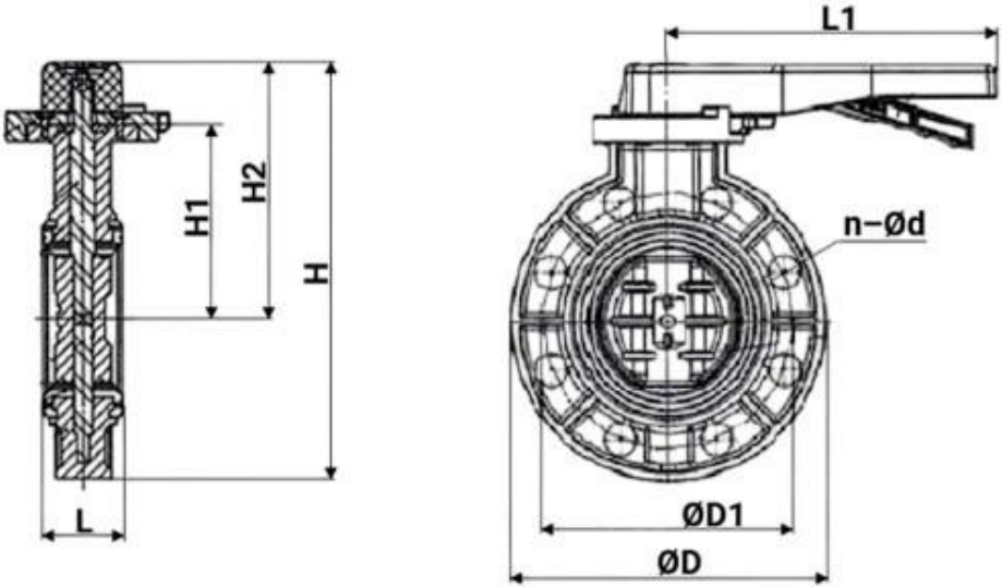
Figure 2 – Dimensions
