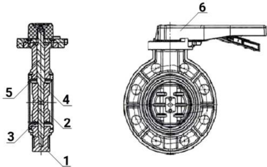
Figure 1 - Detailing
